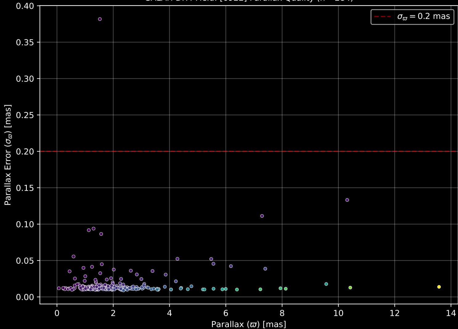
GALAH DR4 Field: [6922] Parallax Quality (n= 284)
