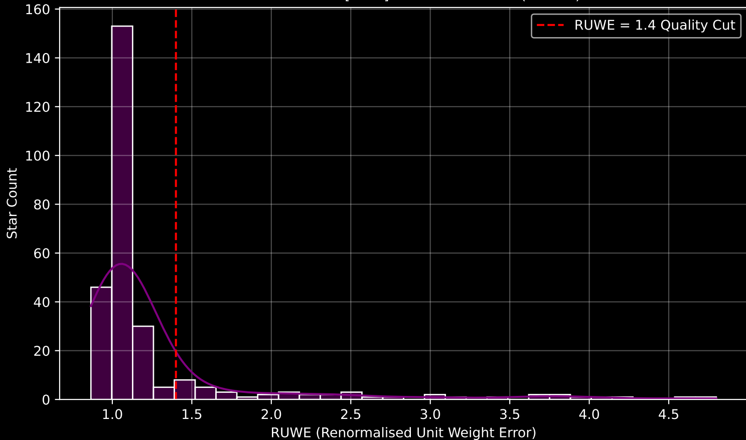
GALAH DR4 Field [6922] RUWE Distribution (n= 278)
