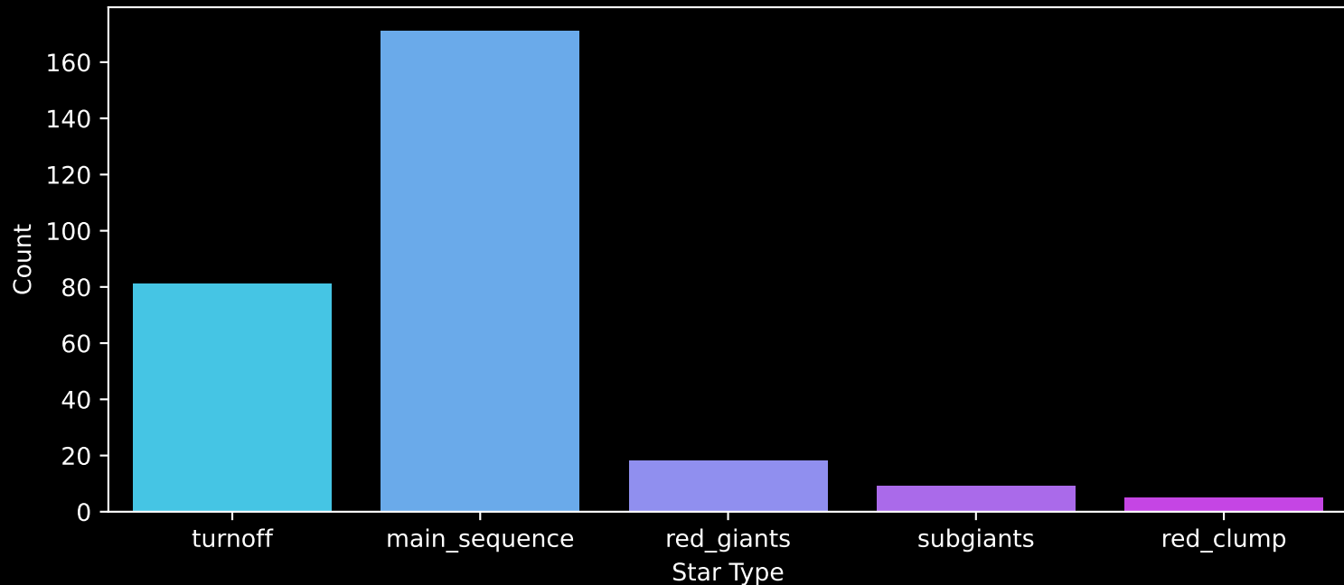
GALAH DR4 Field: [6922] Count plot of Star Type
