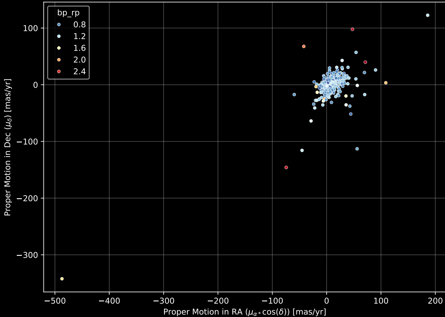
GALAH DR4 Field: [6922] Proper Motion Diagram (n= 284)
